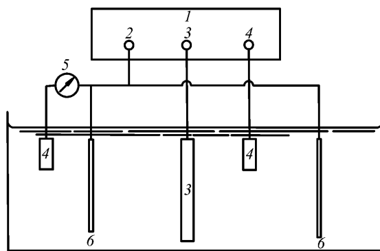
Fig. 2.5.6.1-1 Cathode protective circuit with potentiostatic control:
