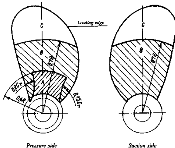
Fig. 2.1 Subdivision of the blade surface into zones: R – propeller radius; C – chord length on radius
