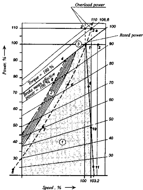
Fig. 8.5 Load points
