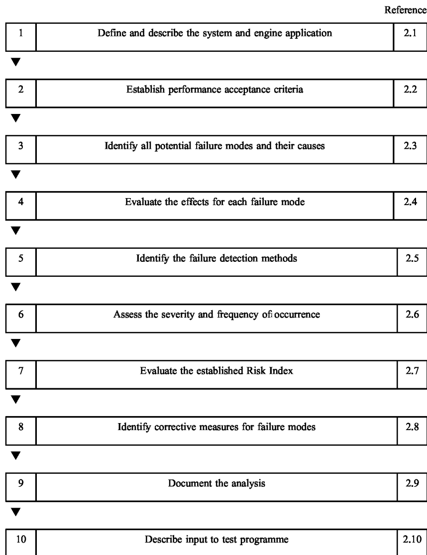
Fig.1. Diesel engine control system FMEA process
