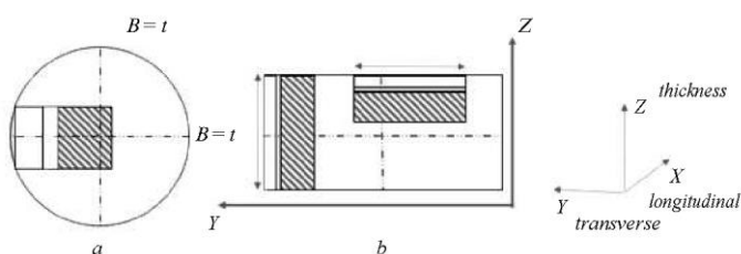
Fig. 7.2.1.6.6 Location of CTOD test specimens: a — circular type accessory; b — rectangular type accessory
