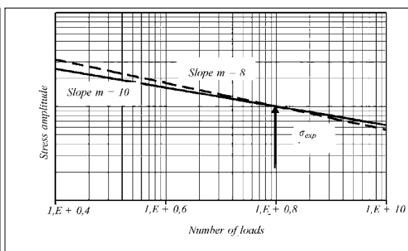
Fig. 10.7.6.2.3-2 Constant-slope SN-curve
