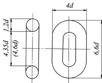
Fig. 7.1.3-3 Studless link
