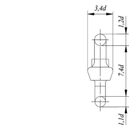
Fig. 7.1.3-5 Joining shackle
