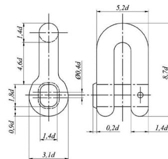
Fig. 7.1.3-6 End shackle
