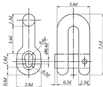
Fig. 7.1.3-5 Joining shackle
