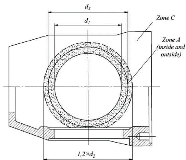
Fig. 4.2.6.2-2 Severity zones for controllible pitch propeller boss
