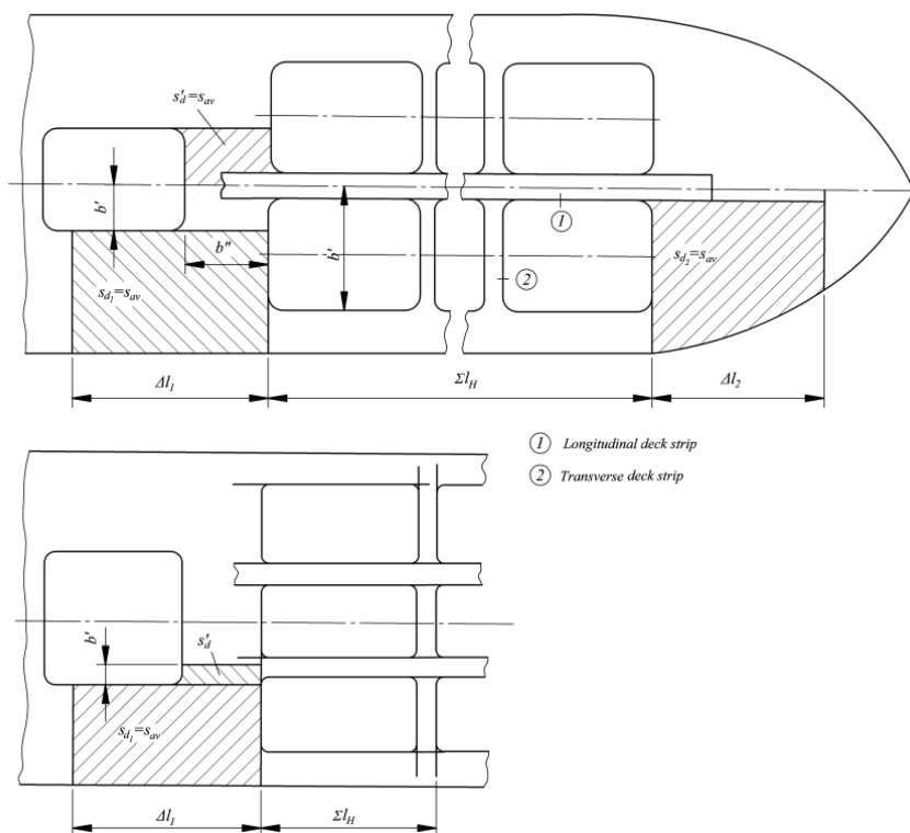
Longitudinal deck strips to be included in the calculation of hull section modulus
