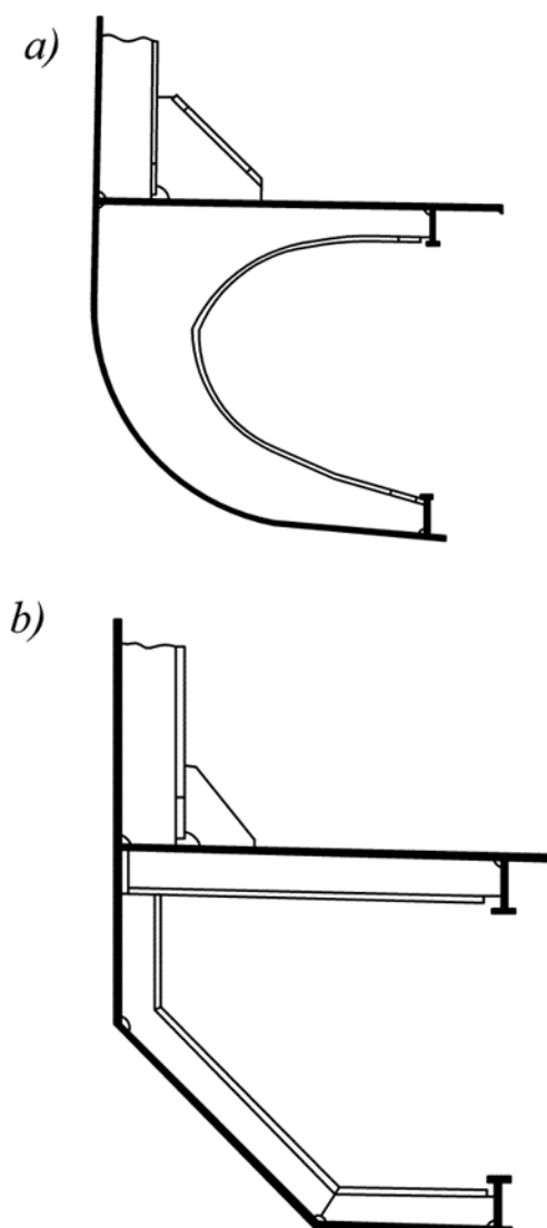
Fig. 3.10.2.1.3-1: a — lightened margin bracket; b — system of stiffeners
