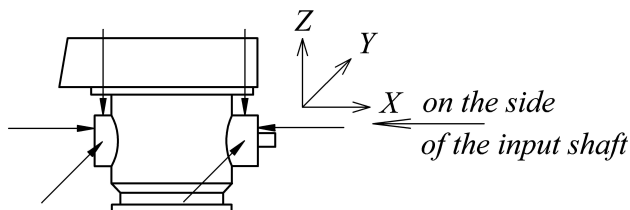
Fig. 9.9.2 Points of vibration measuring of azimuth thrusters
