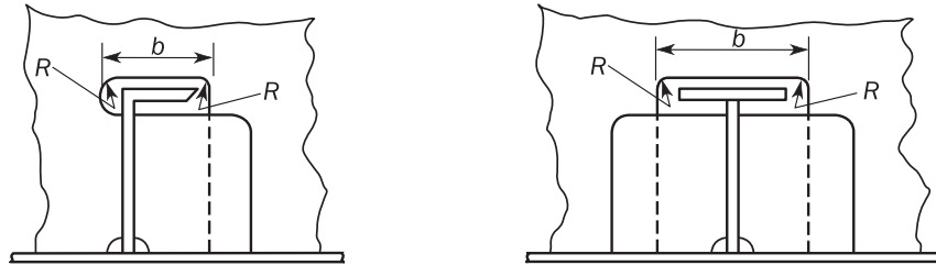
Figure 7 : Full collar plates
