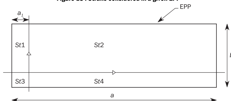
Figure 18 : Strake considered in a given EPP
