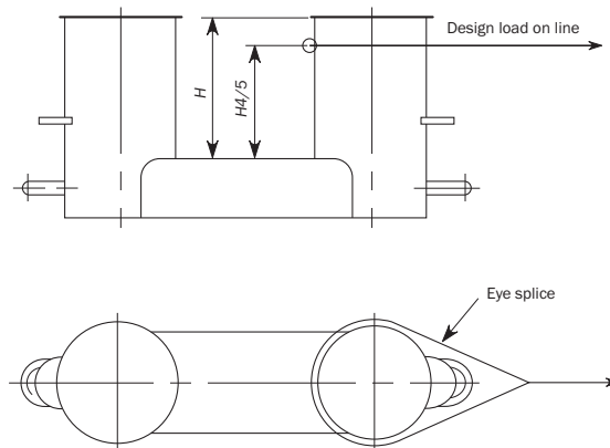
Figure 5 : Attachment point of the towing line
