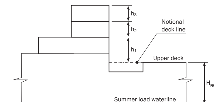
Figure 1 : Measurement of heights
