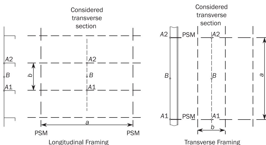
Figure 23 : LCP for plate buckling - hull girder stresses
