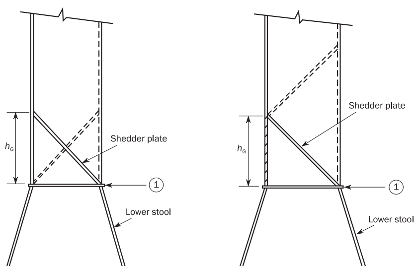
Figure 5 : Symmetrical and unsymmetrical gusset / shedder plates
