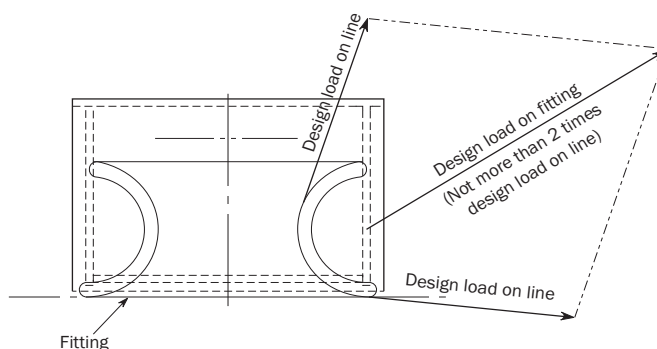
Figure 4 : Design load on fitting
