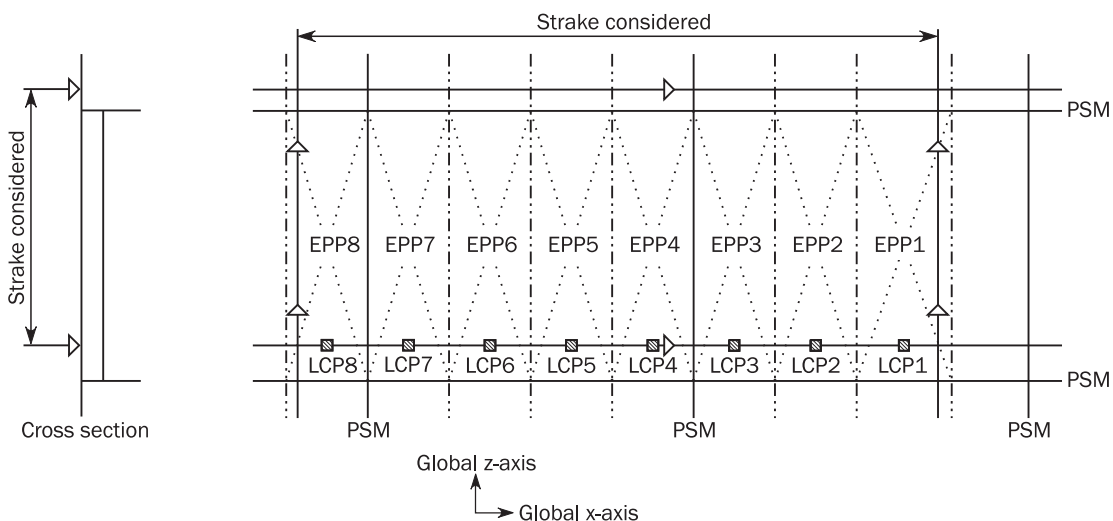
Figure 20 : Load calculation point for transverse framing
