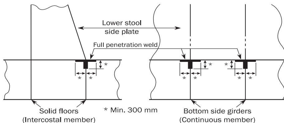
Figure 3 : High stress areas welding (examples)
