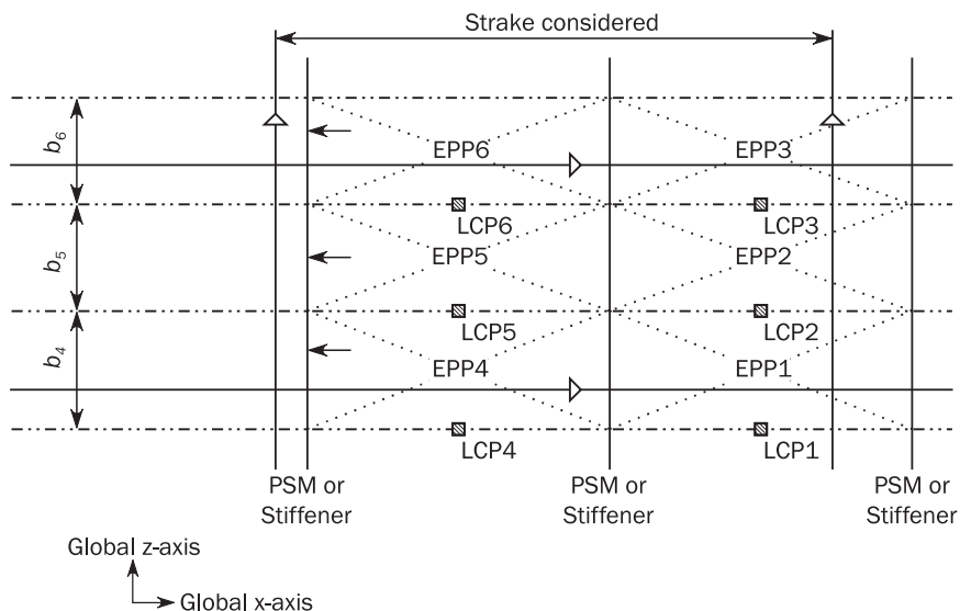
Figure 19 : Load calculation point (LCP) for longitudinal framing
