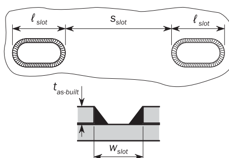
Figure 9 : Slot welds
