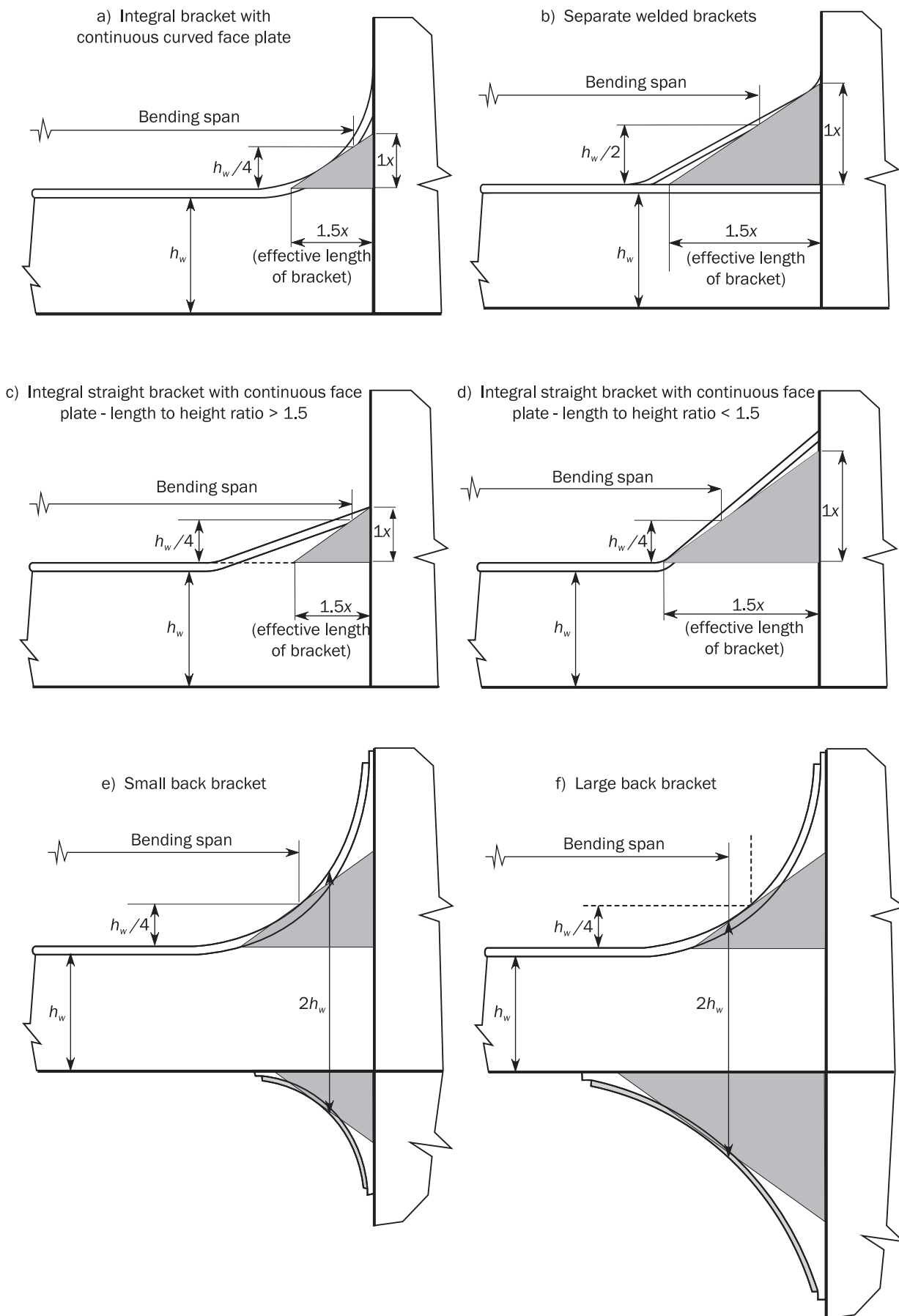
Figure 9 : Effective bending span of primary supporting member
