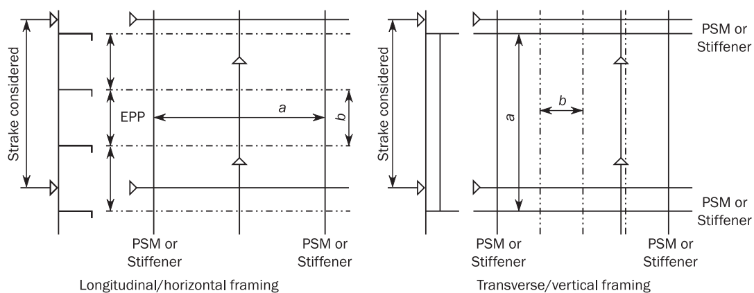
Figure 17 : Elementary Plate Panel (EPP) definition
