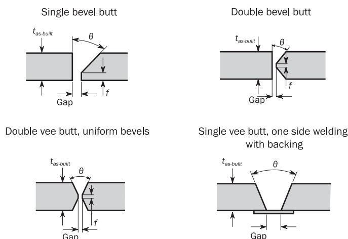
Figure 7 : Typical butt welds
