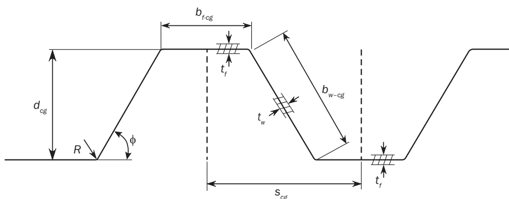
Figure 21 : Dimensions of a corrugated bulkhead
