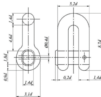
Fig. 7.1.3-6 End shackle
