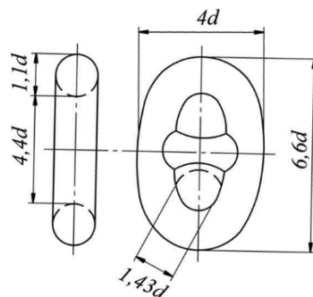
Fig. 7.1.3-2 Enlarged link
