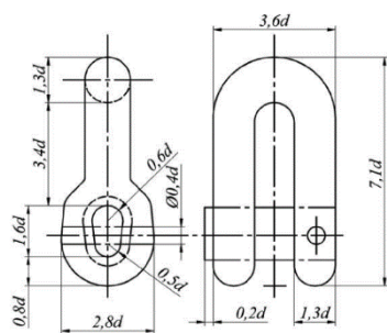
Fig. 7.1.3-5 Joining shackle
