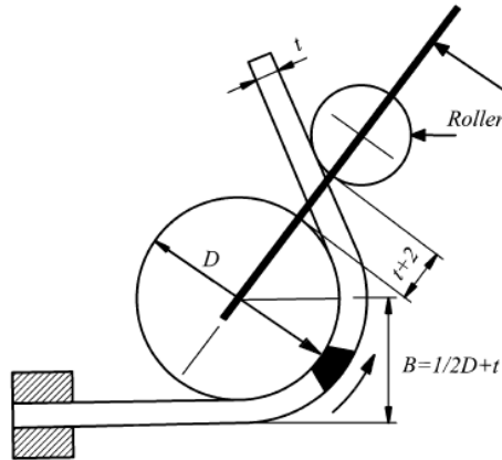
Fig. 4.9.3.6 Sketch of wrap around bend test
