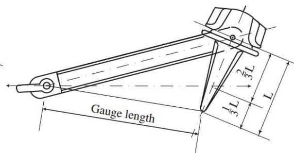
Stocked Anchor
