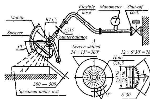
Fig. 5.2-2 Portable set-up for checking the protection against rain and spraying with water (sprayer), dimensions are given in mm
