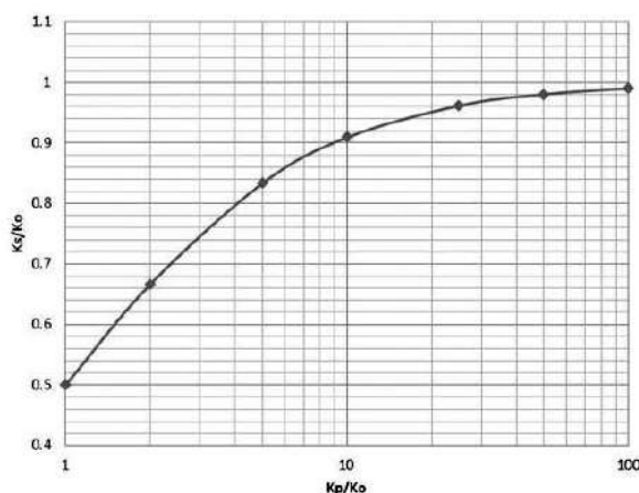
Fig. 1.2.5 Relation between bearing stiffness and support
