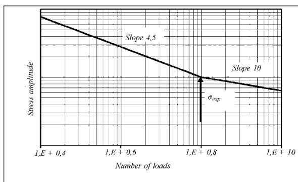
Fig. 10.7.6.2.3-1 Two-slope SN-curve
