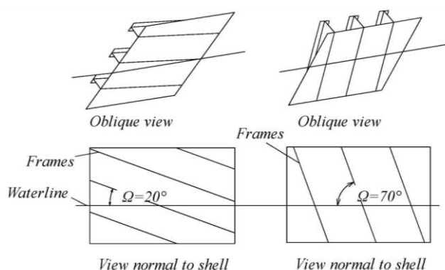
Fig. 1.2.4.2 Shell framing angle \Omega
